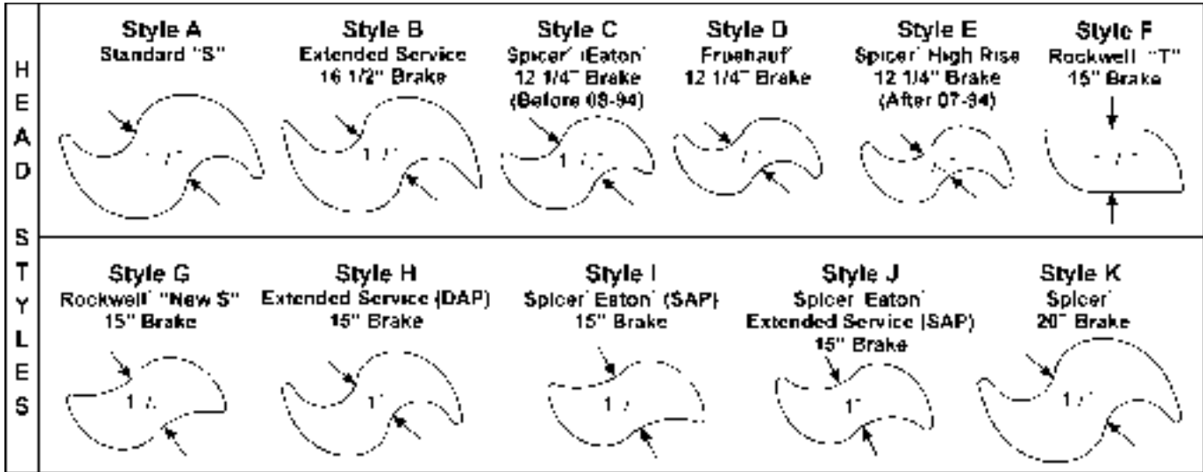
These graphics are for identification purposes only. Dimensions in actual camshafts may vary slightly.
